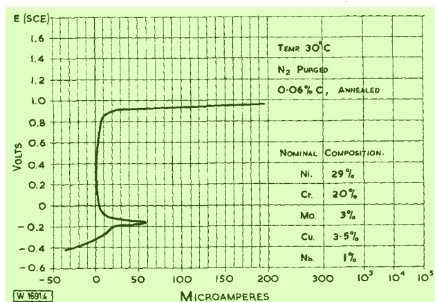
Fig. 4. Polarisation characteristics of LINGALLOY 20V special stainless steel in 1 N H 2 SO 4
