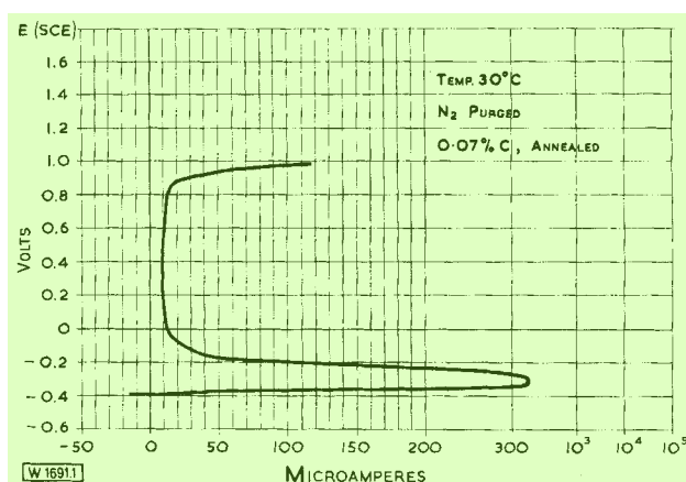
Fig. 1. Polarisation characteristics of 18Cr10Ni in 1 N H 2 SO 4 7
