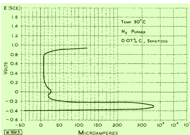
Fig. 5. Polarisation characteristics of 18Cr10Ni in 1 N H 2 SO 4
