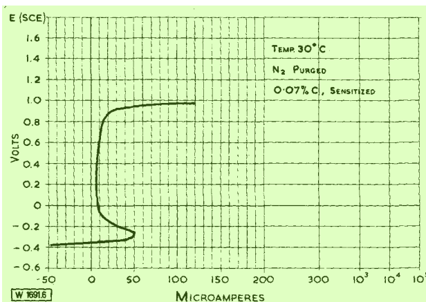
Fig. 6. Polarisation characteristics of 18Cr10Ni3Mo in 1 N H 2 SO 4
