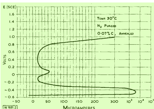
Fig. 2. Polarisation characteristics of 17 Cr ferritic steel in 1 N H 2 SO 4 14
